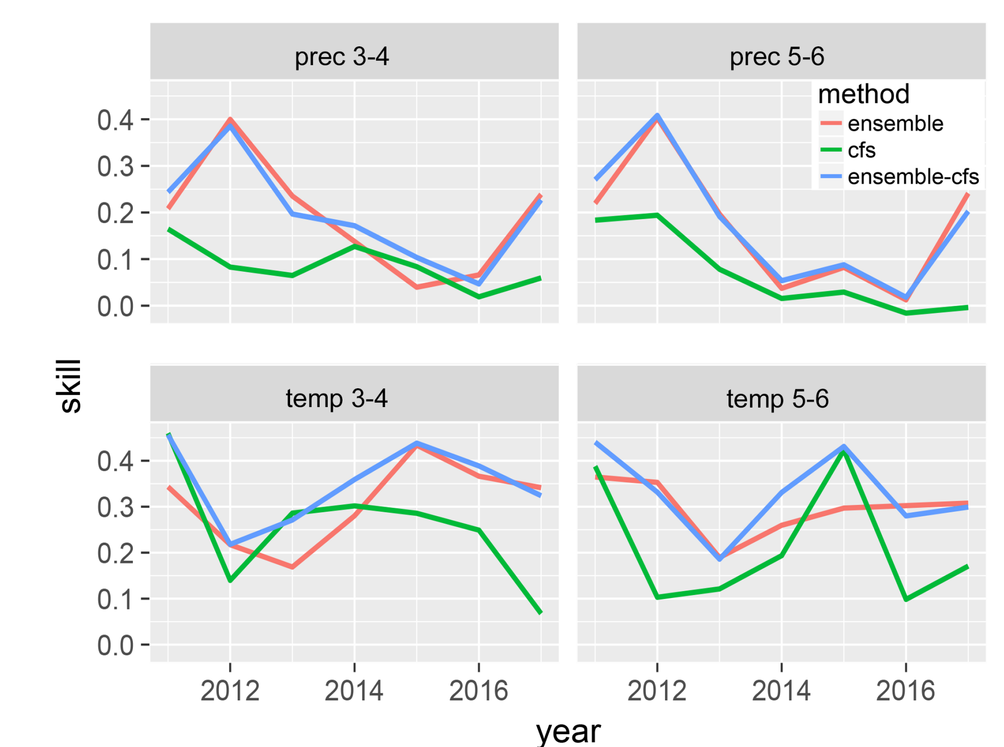
Fig 4: Performance of ens, cfs, and ens-cfs in the historical period.
