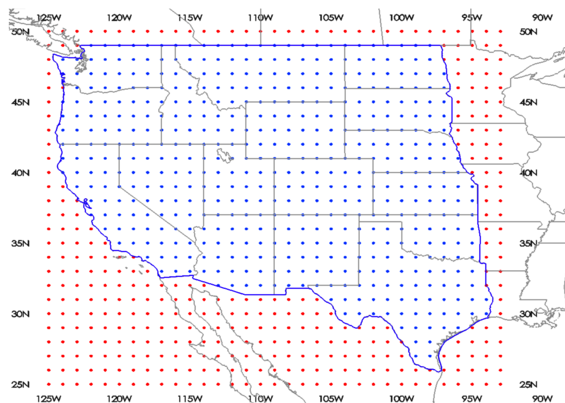
Fig 1: Forecast Rodeo prediction region.
