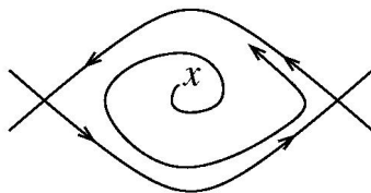
Fig. 1. A system without time-averages
