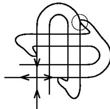
Fig. 2. A homoclinic tangency
