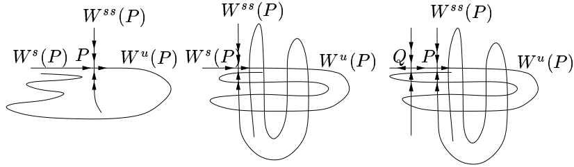
FIGURE 2. Saddle-node cycles
