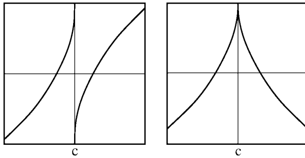
Figure 2: One-dimensional return map
