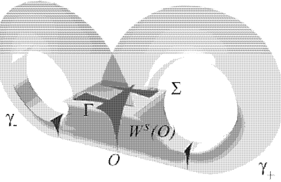
Figure 1: Geometric Lorenz attractor
